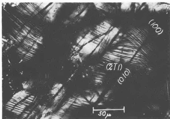
Fig. 1. Andesine in dioritic gneiss, Zipplingen. Isotropic slip bands (black) are parallel to (100) and (\bar{2}\bar{1}1) ; isotropic twin lamellae (black) are parallel to (010). Irregular isotropic areas (black) are present. Crossed nicols.
