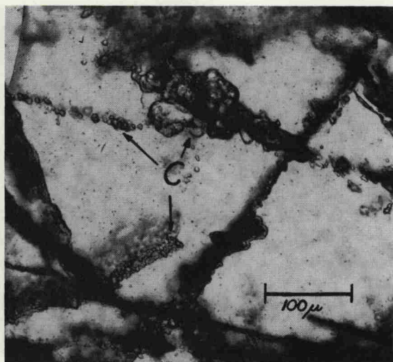
Fig. 3. Diaplectic quartz glass (light areas) with aggregates of fine-grained coesite (C) within a fragment of biotite granite from Aufhausen.
